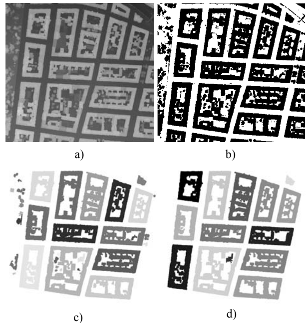
Figure 2. Building detection in a test site in the City of Vienna. Original resolution: 0.1 m (in-flight) by 1 m (cross-flight). a) DSM; grid width: 0.5 x 0.5 m 2 ; extent: 410 x 435 m 2 . b) Initial building mask (height threshold \Delta h_{\min}=3.5\text{m} ). c) initial building label image before evaluating terrain roughness. d) Final building label image.
