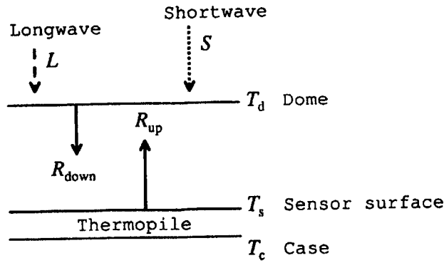
Figure 1. Schematic diagram of energy balance for PIR or PSP. L is the longwave irradiance from a target; S is the shortwave irradiance; R_{\text{down}} and R_{\text{up}} are the downward and the upward irradiances between the dome and the thermopile. T_c , T_d , and T_s are the temperature of the case, the dome, and at the upper surface of the thermopile, respectively.
