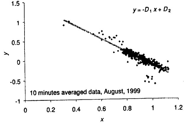
Figure 4. Nighttime field measurements of two PIRs plotted by using Eq. (7). Linear relationship between x and y is expected for an equilibrium system.
