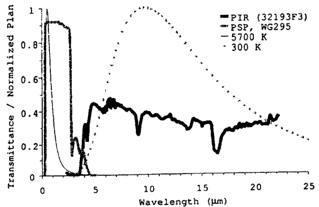
Figure 2. Transmittance of a PSP dome (Schott Glass Technologies Inc., long pass filter WG 295) and a PIR dome (silicon dome with interference filter, SN 32193F3). The normalized Planck functions at 5700 K and at 300 K are also shown.
