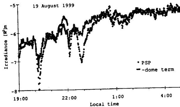
Figure 5. Nighttime measurements of a PSP (32188F3) comparing to the calculated values based on the thermal dome effect term in Eq. (8).
