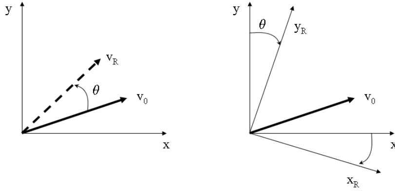
Figure A.3: Active (Left) vs. Passive (Right) Rotation
