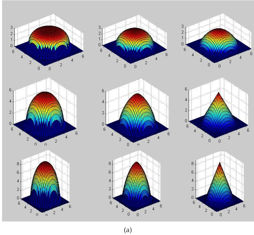
Figure 4.18: Various shapes represented by the tree model. b = 3 in all cases. Top row: a = 3, n = 4, 3, 2 . Middle row: a = 6, n = 2, 1.5, 1 . Last row: a = 8, n = 2, 1.5, 1 .
