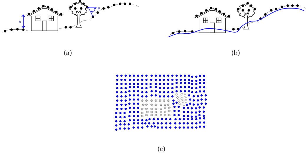
Figure 4.4: Methods of DTM extraction: (a) Local region-based, (b) Function-based, and (c) Feature/segmentation-based.
