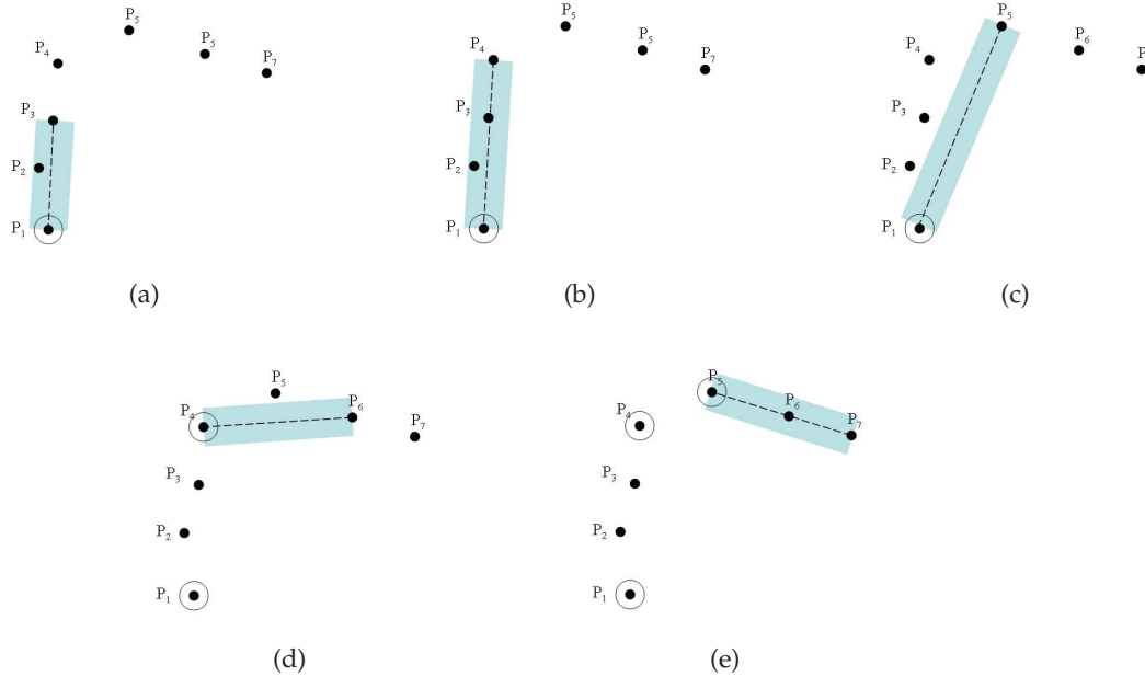
Figure 4.23: The sleeve method: (a) P_2 falls within the sleeve defined by P_1 and P_3 , (b) P_2 and P_3 fall within the sleeve defined by P_1 and P_4 , (c) Points fall outside the sleeve defined by P_1 and P_5 ; P_4 identified as a critical point, (d) P_5 falls outside the sleeve identified by P_4 and P_6 ; P_5 identified as a critical point, (e) The process continues around the set of boundary points.
