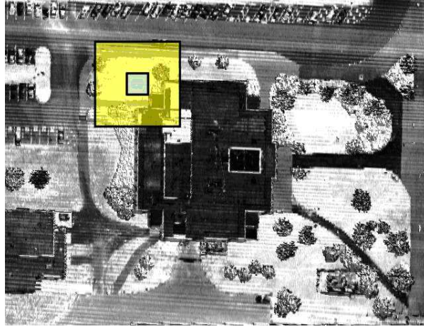
Figure 4.6: Illustration of the Modified Minimum Filter at a single location; minimum height value is calculated in smaller window, points 3m above minimum in larger window are flagged as non-ground points.
