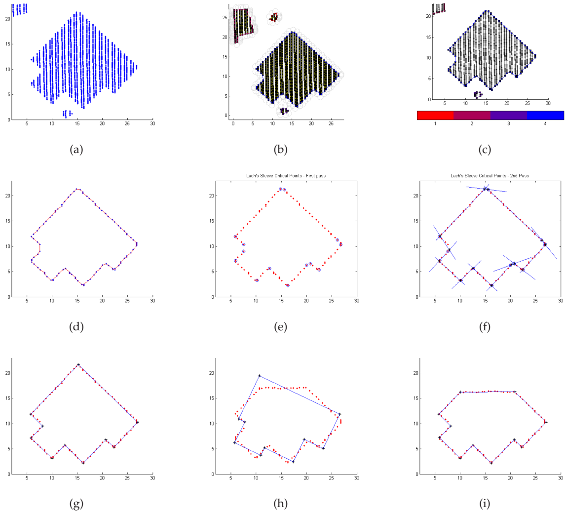
Figure 4.26: Illustration of the boundary extraction process.
